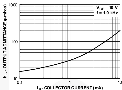
Figure 20. Output Admittance
