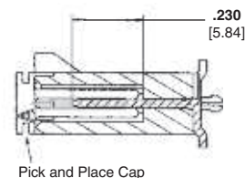
Section K-K
