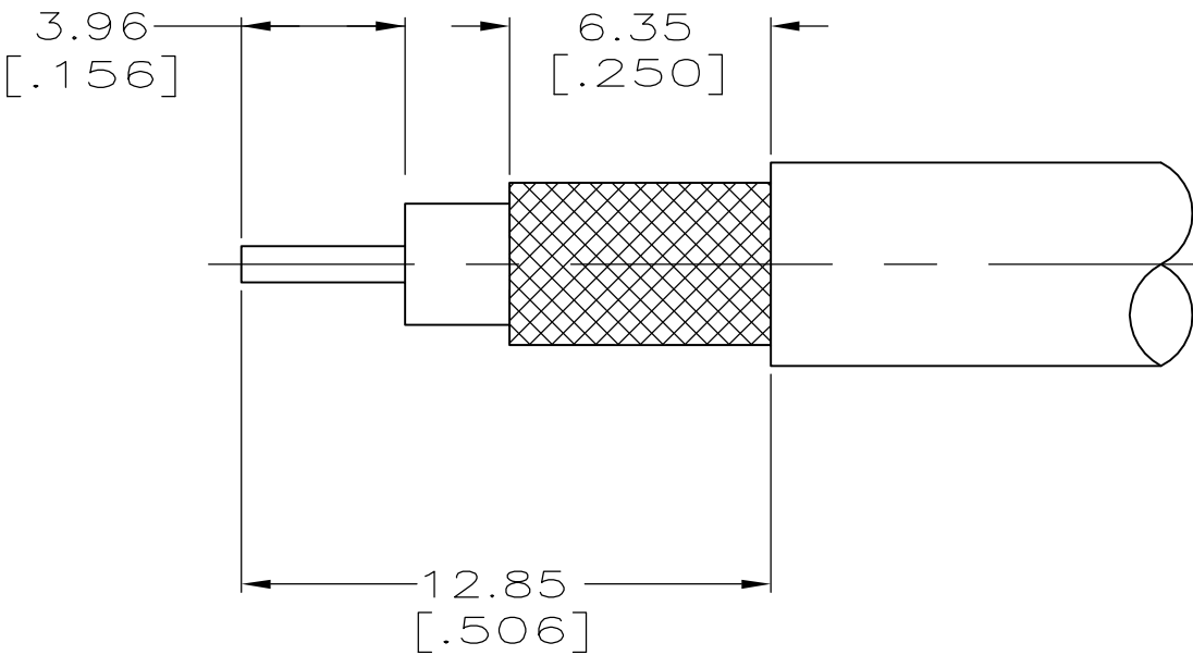
VIEW B
