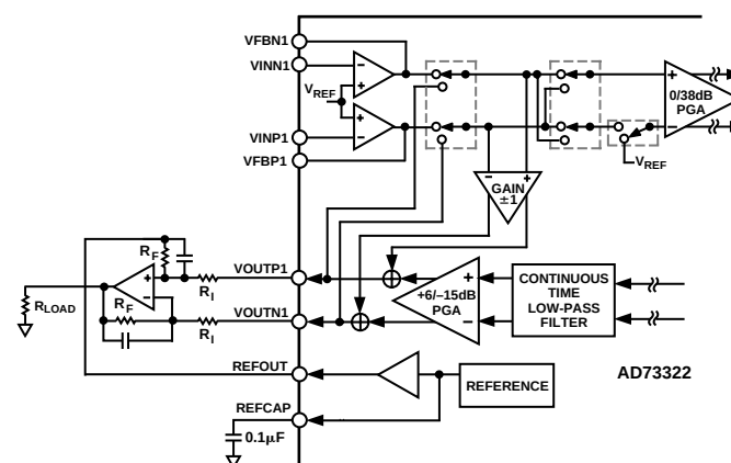
Figure 37. Example Circuit for Differential to Single-Ended Output Conversion
