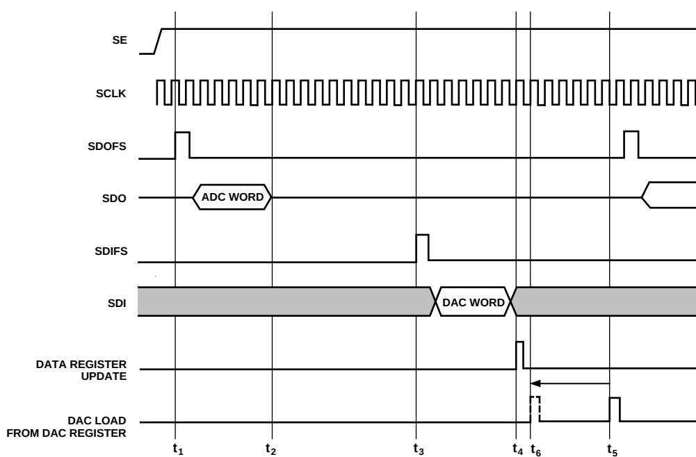
Figure 43. DAC Timing Control
