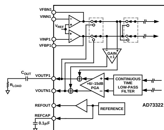
Figure 36. Example Circuit for Single-Ended Output
