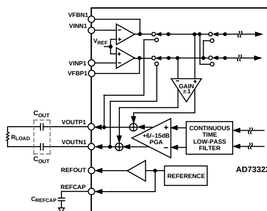
Figure 35. Example Circuit for Differential Output
