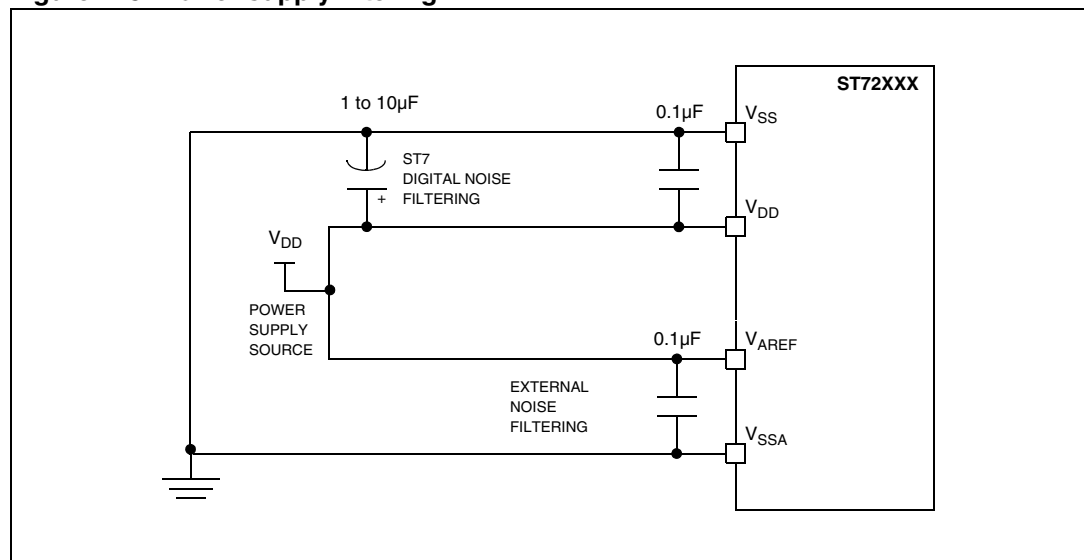
Figure 115. Power supply filtering
