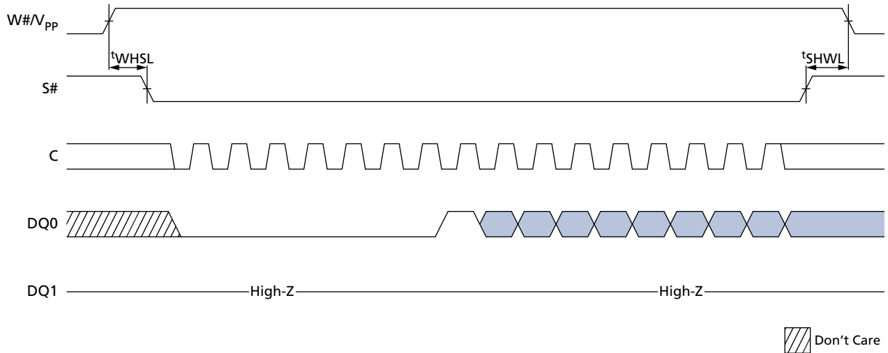
Figure 36: Hold Timing
