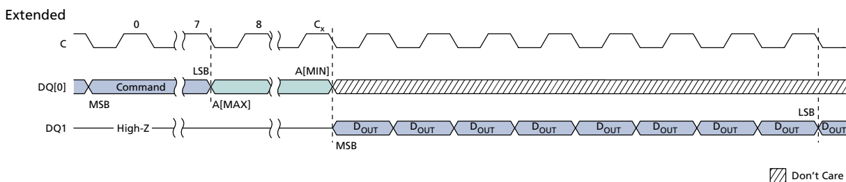
Figure 13: READ Command
