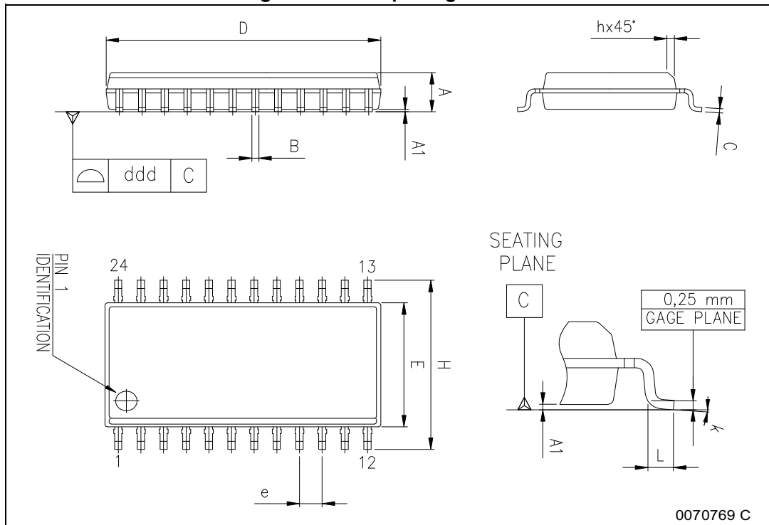
Figure 31. SO24 package outline
