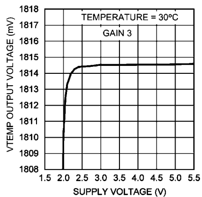
V TEMP vs. Supply Voltage Gain 3: For Trip Points 110 - 129°C
