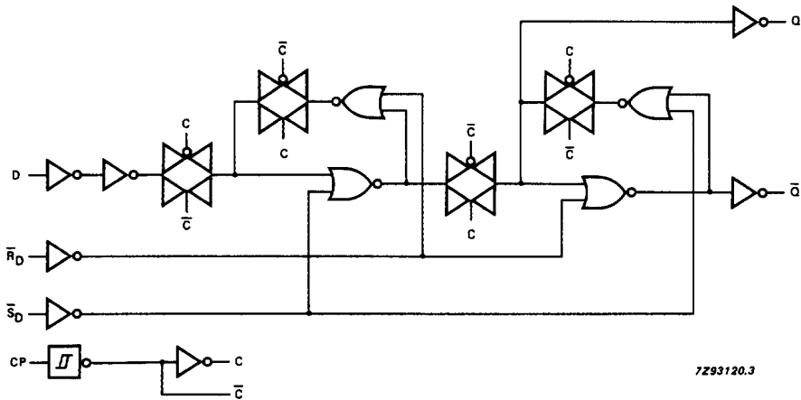
Fig.5 Logic diagram (one flip-flop).
