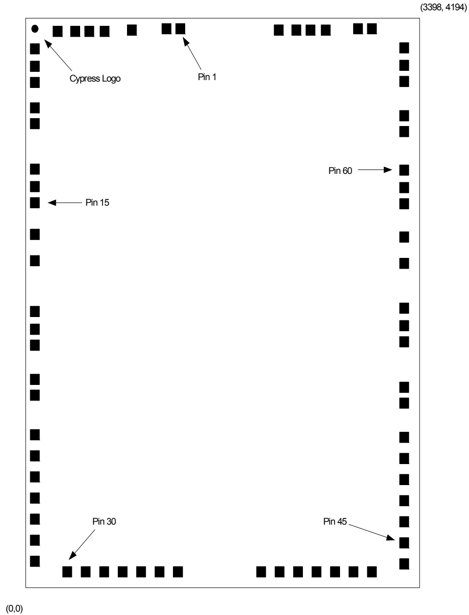
Figure 3. CY7C66113C DIE
