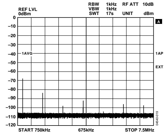
Figure 11. THD @ 400 MSPS and f_{OUT} = 1 MHz (Diplexer High-Pass Output Showing Harmonics Before Calibration; See Performance Effects of Calibration Section)
