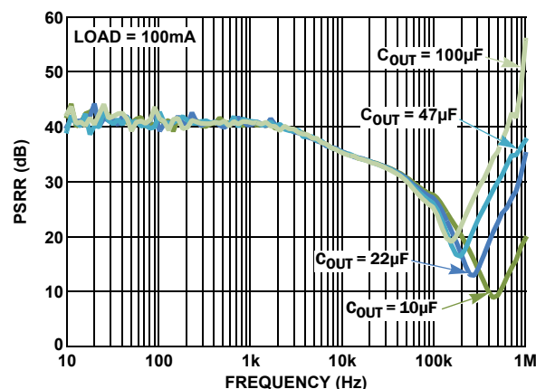
FIGURE 12. PSRR vs FREQUENCY FOR VARIOUS OUTPUT CAPACITORS ( I_{OUT} = 100mA )
