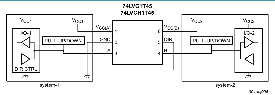
Fig. 13. Bidirectional logic level-shifting application
