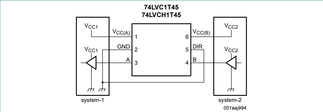
Fig. 12. Unidirectional logic level-shifting application
