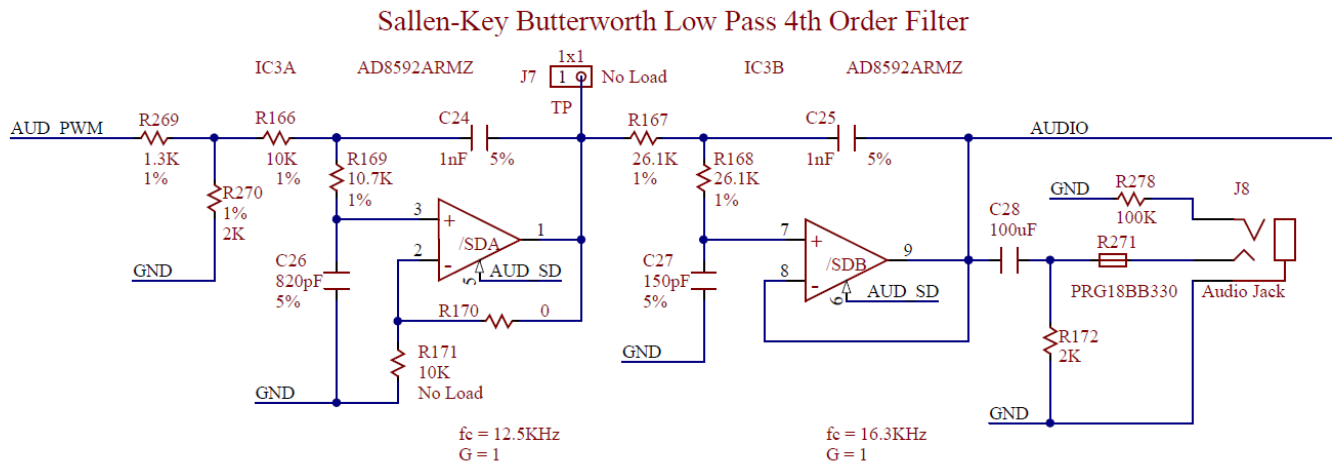
Figure 29. Sallen-Key Butterworth Low Pass 4 th Order Filter
