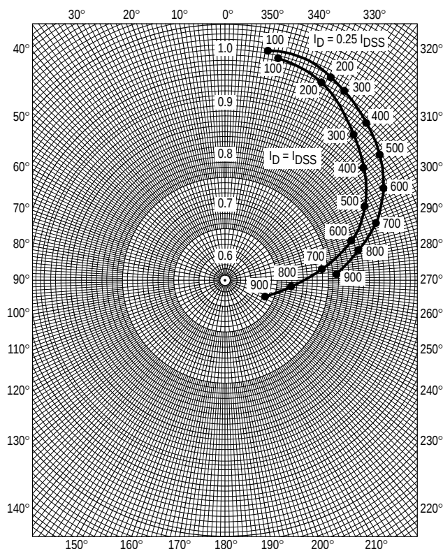
Figure 10. S_{11s}
