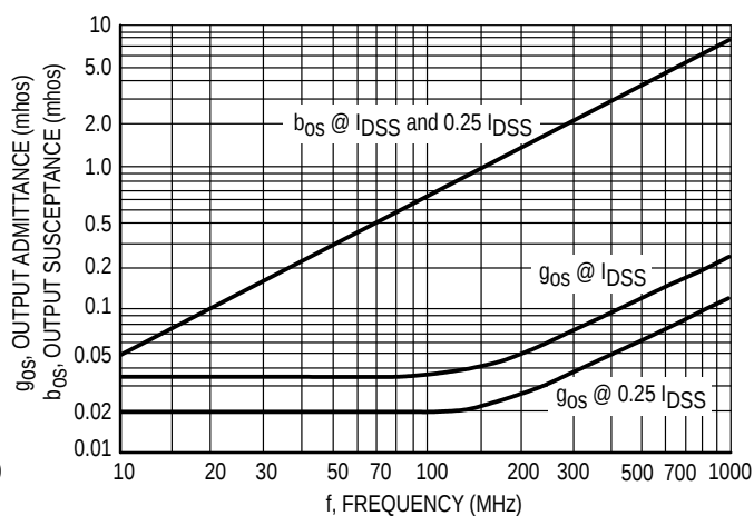
Figure 9. Output Admittance ( y_{os} )
