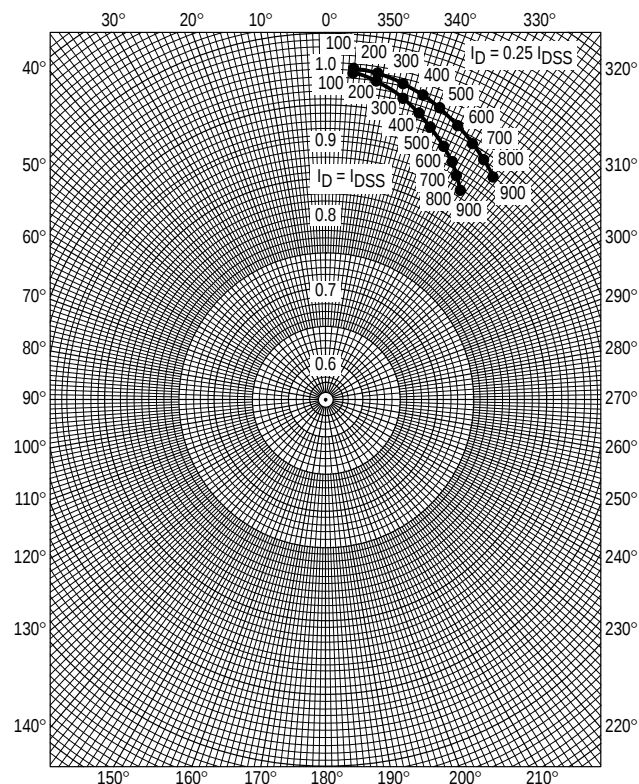
Figure 13. S_{22s}
