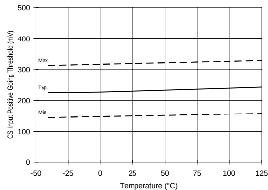
Figure 16A. CS Input Threshold (+) vs. Temperature
