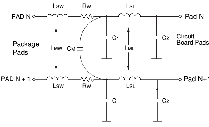
Figure 102. Package Parasitics
