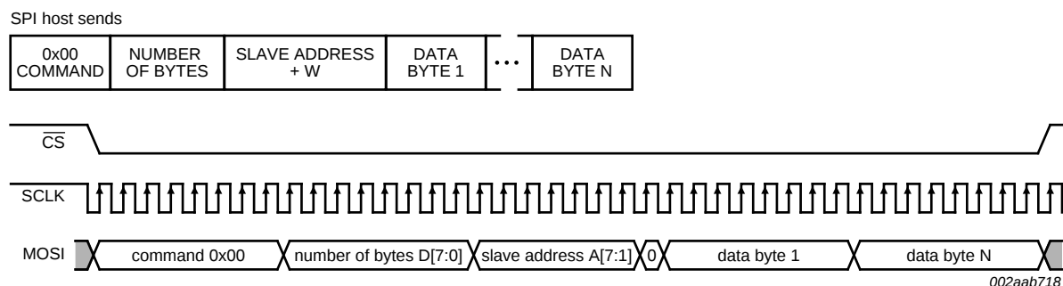
Fig 11. Write N bytes to I 2 C-bus slave device
