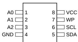
8-lead SOIC
