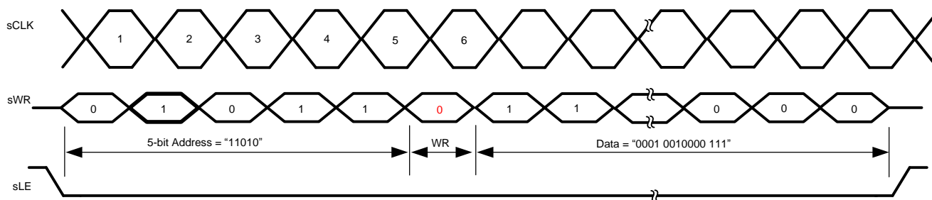
Figure 17. Write Register 1Ah with 14 bit = 0001 0010000 111
