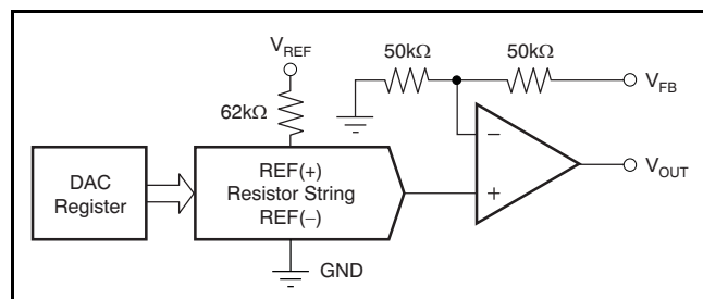
Figure 45. DAC8550 Architecture
