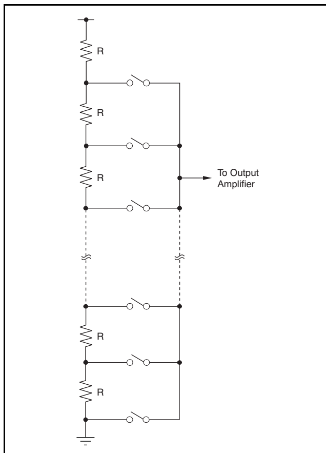
Figure 46. Resistor String
