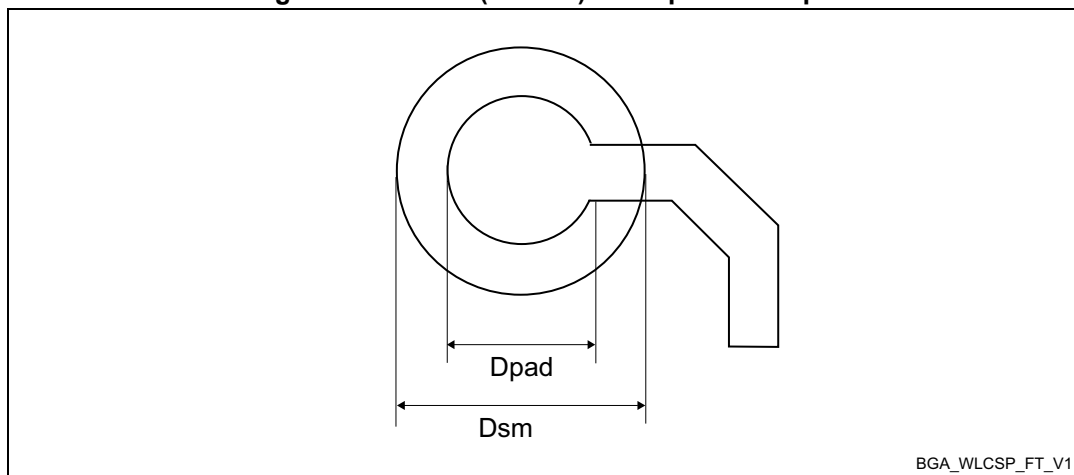
Figure 89. UFBGA(176+25) - Footprint example
