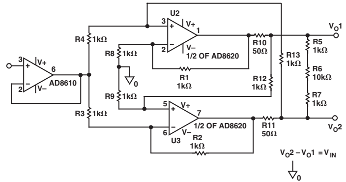
Figure 30. Differential Driver
