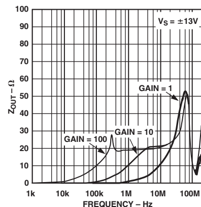
TPC 27. Z_{OUT} vs. Frequency
