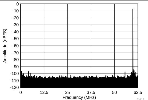
Figure 46. FFT for Two-Tone Input Signal (-7 dBFS at 185 MHz and 190 MHz)
