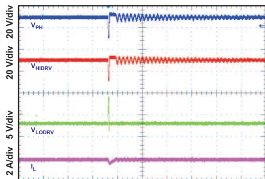
NEAR 100% DUTY CYCLE BOOTSTRAP RECHARGE PULSE
