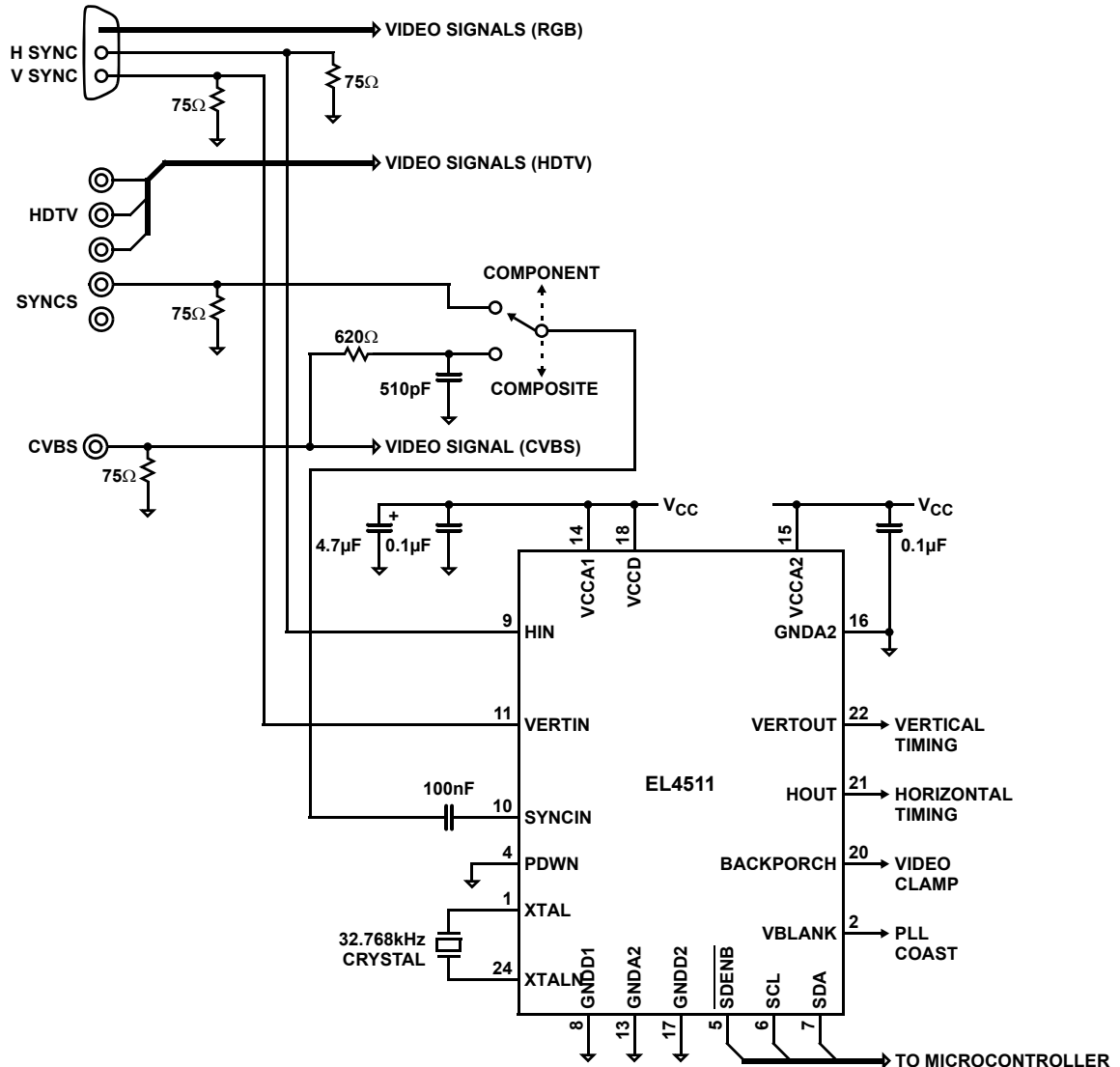
FIGURE 12. APPLICATIONS DRAWING 3
