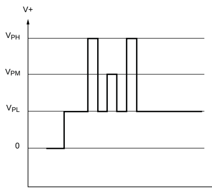
Figure 7. Addressing mode enable pulse sequence
