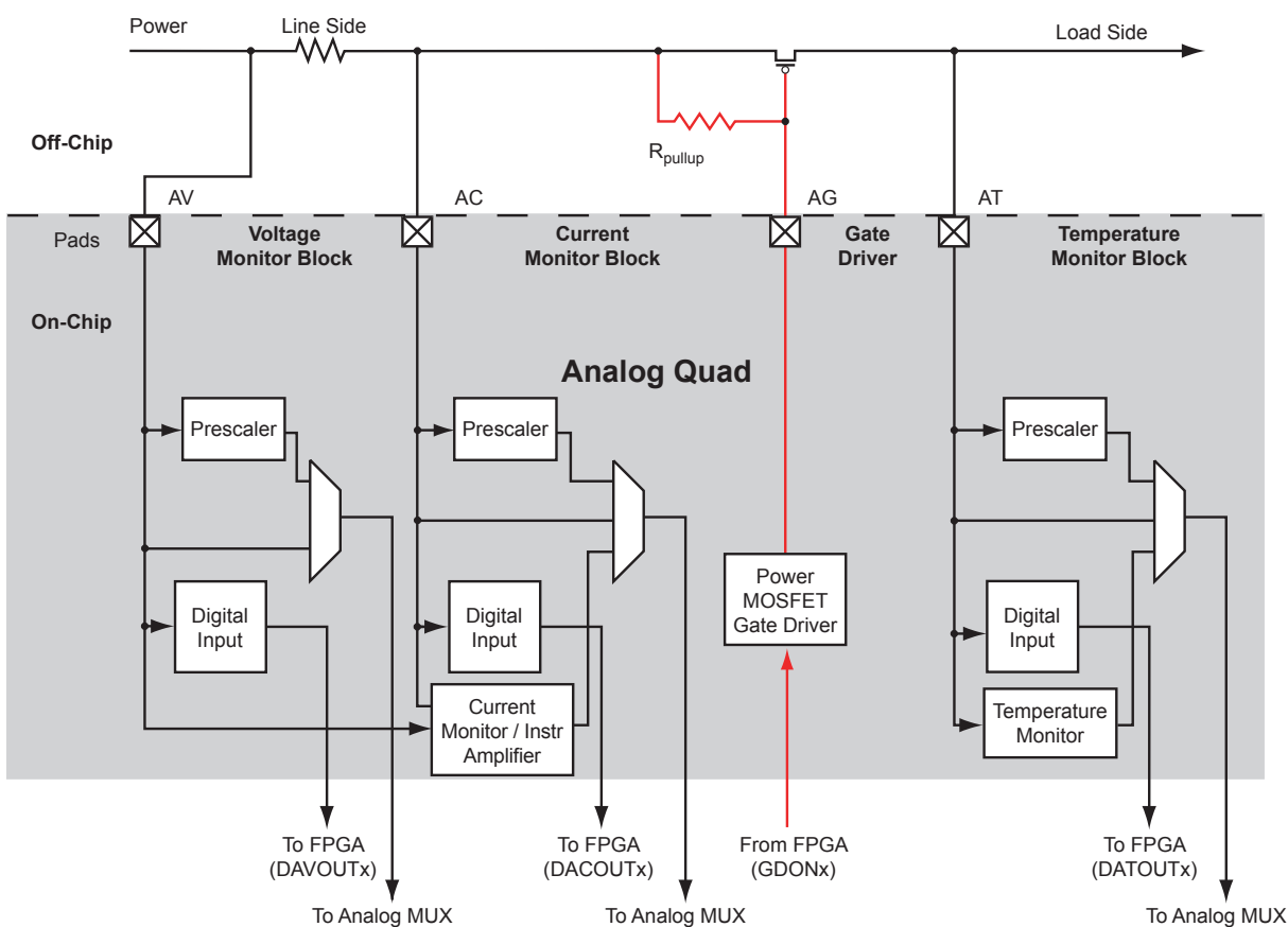
Figure 2-74 • Gate Driver
