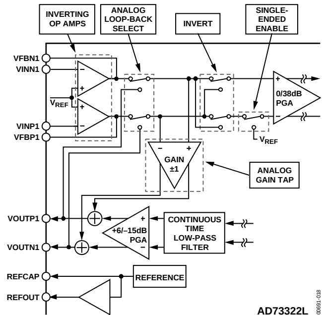
Figure 18. Analog Input/Output Section
