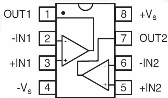
Figure 5. FAN4274 MSOP
