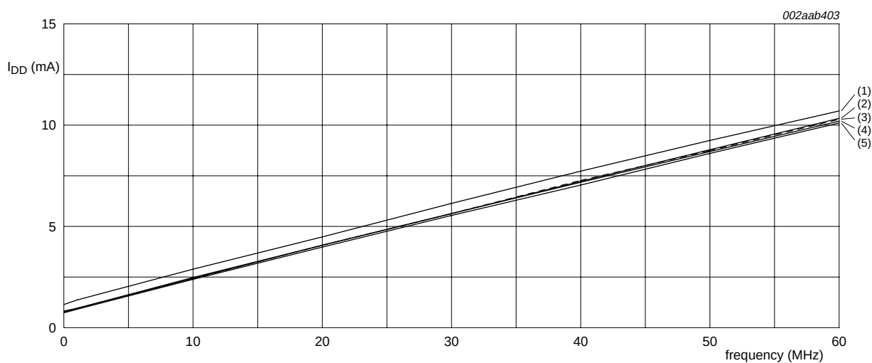
Fig 11. I_{DD} idle measured at different frequencies (CCLK) and temperatures
