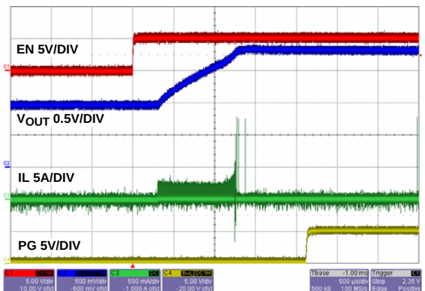
FIGURE 26. SOFT-START WITH PRE-BIASED V_1
