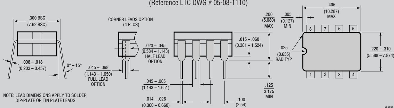
J8 Package 8-Lead CERPDP (Narrow .300 Inch, Hermetic) (Reference LTC DWG # 05-08-1110)
