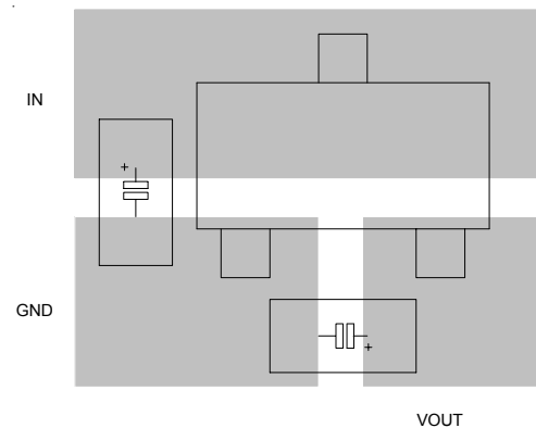
SOT-23 Board Layout
