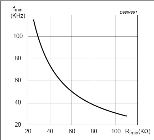
Figure 8. Typ. f_{min} vs. R_{fmin} at C_f = 470 pF
