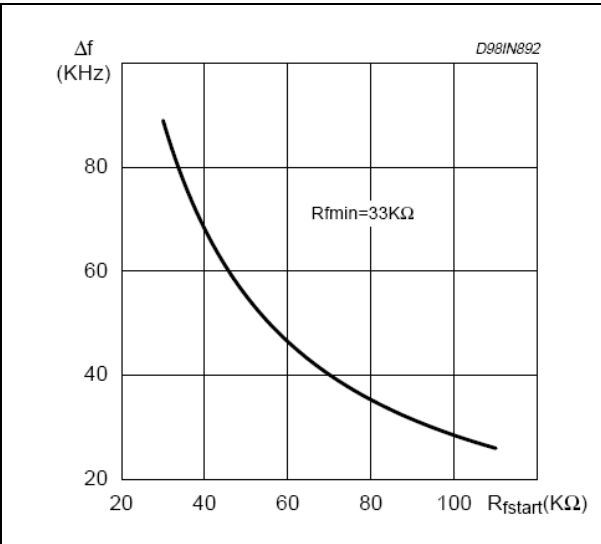
Figure 10. Typ. (f_{start}-f_{min}) vs. R_{fstar} at C_f = 470 pF
