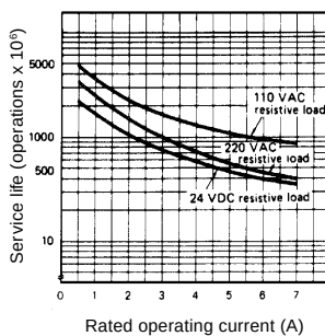
MY2-Y(Resistive load)
