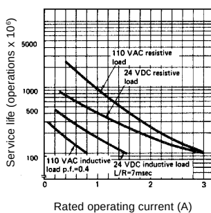
MY2-Y(Resistive load)
