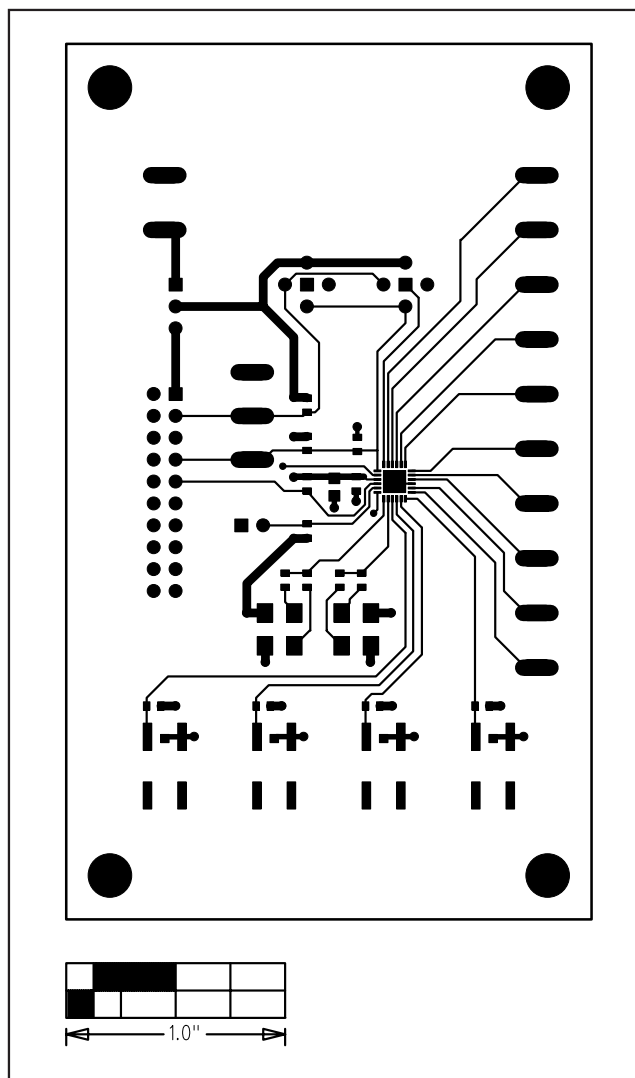
Figure 4. MAX7326 EV Kit PCB Layout—Component Side
