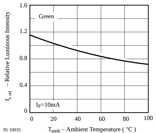
Figure 21 Rel. Luminous Intensity vs. Ambient Temperature
