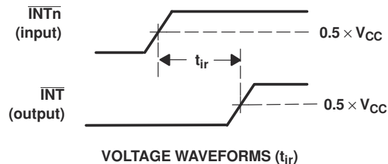
Figure 7-3. Interrupt Load Circuit and Voltage Waveforms
