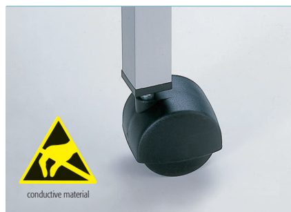
Art. No. EGB-Rollboy Single 4 with 18 drawers (cf. inside dimensions drawers page 81) Outside dimensions 318 x 365 x 806 Note Please order inserts separately conductive pad on request
