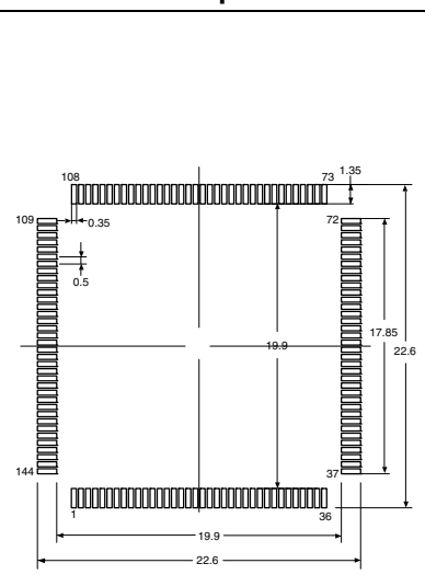
Figure 39. Recommended footprint
