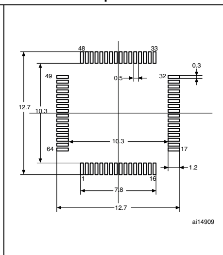
Figure 43. Recommended footprint
