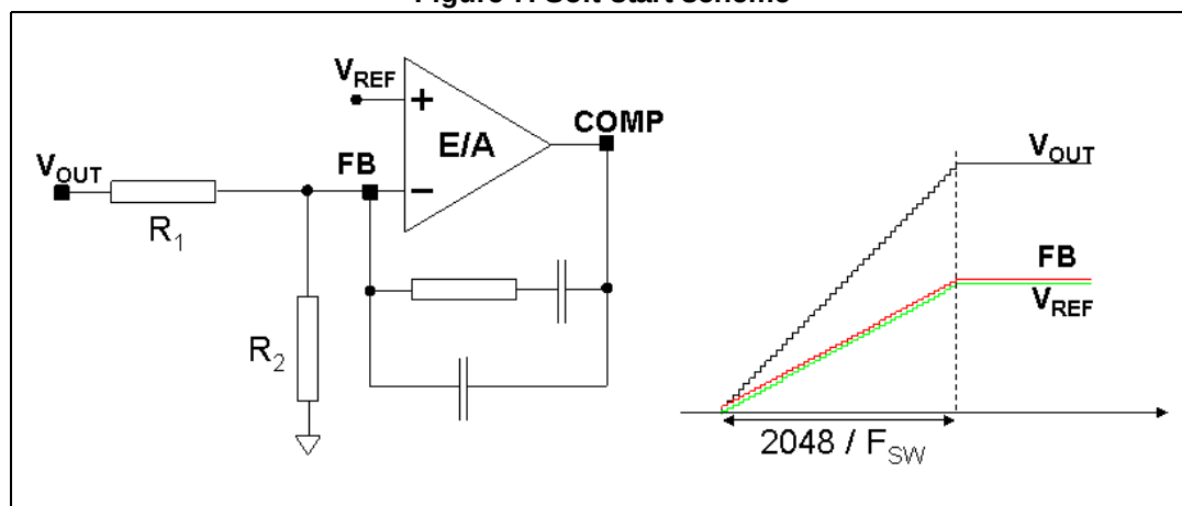
Figure 7. Soft-start scheme
