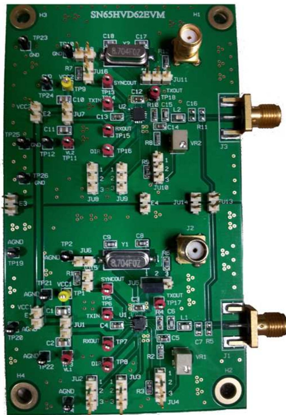
Figure 2. SN65HVD62 EVM
