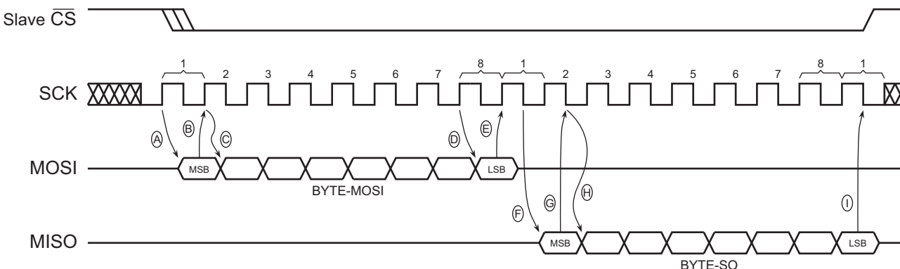
Figure 19-1. RapidS Mode
