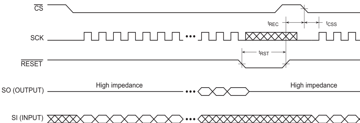
Figure 19-2. Reset Timing
