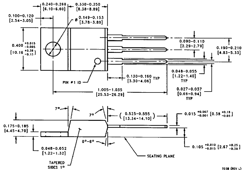
3-Lead TO-220 Package Order Part Number LM3940IT-3.3 NSC Package Number TO3B
