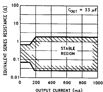
FIGURE 1. ESR Limits
