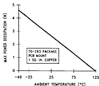
FIGURE 4. Maximum Power Dissipation vs T_{AMB} for the TO-263 Package
