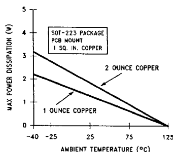
FIGURE 6. Maximum Power Dissipation vs T_{AMB} for the SOT-223 Package
