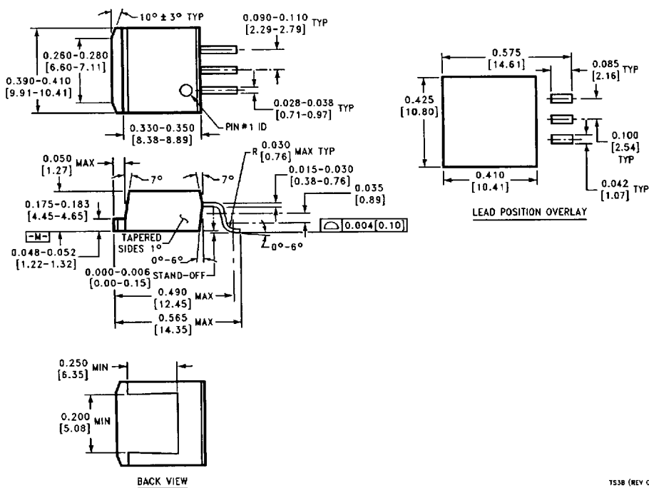
3-Lead TO-263 Package Order Part Number LM3940IS-3.3 NSC Package Number TS3B
