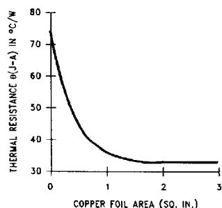
FIGURE 3. \theta_{(J-A)} vs Copper (1 ounce) Area for the TO-263 Package
