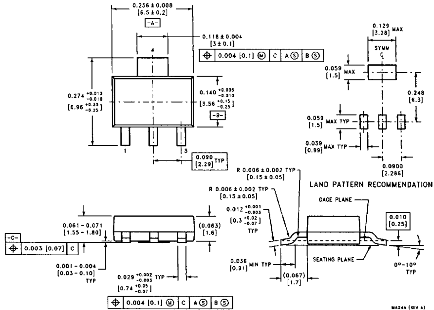
3-Lead SOT-223 Package Order Part Number LM3940IMP-3.3 NSC Package Number MA04A
