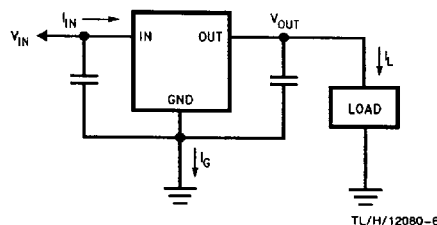
FIGURE 2. Power Dissipation Diagram
