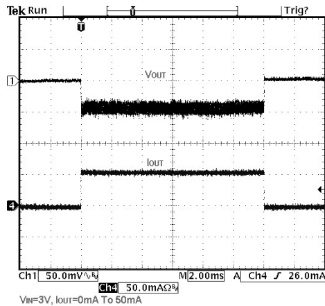
Load Transient for 50mA
