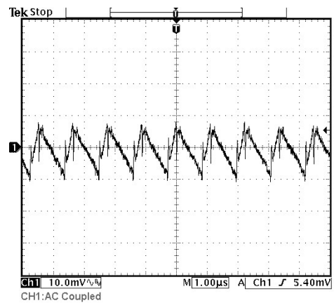
Output Ripple with I_{OUT}=90mA
