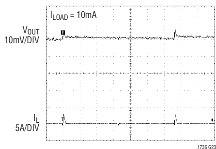
V_{OUT(RIPPLE)} (Synchronized)
