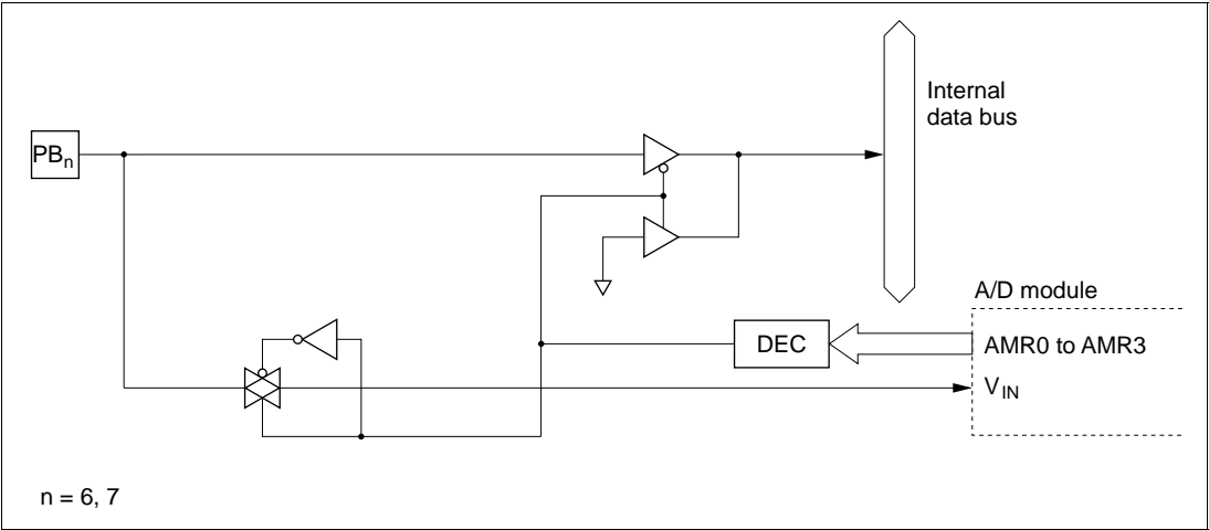
Figure C.8 Port B Block Diagram
