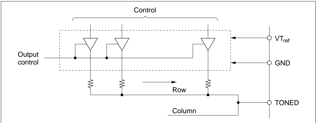
Figure 11.3 Equivalent Circuit for TONED Output
