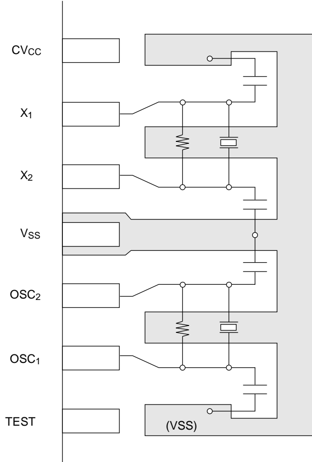
Figure 4.10 Example of Crystal and Ceramic Oscillator Layout.
