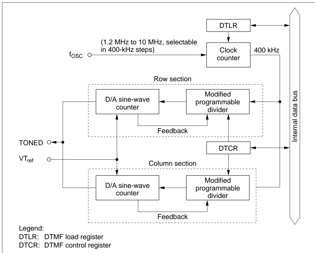
Figure 11.2 DTMF Generator Block Diagram
