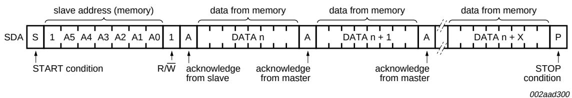
Fig 16. Sequential read
