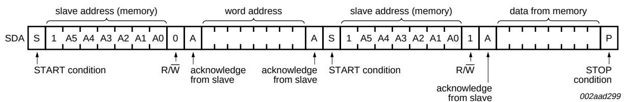
Fig 15. Random read
