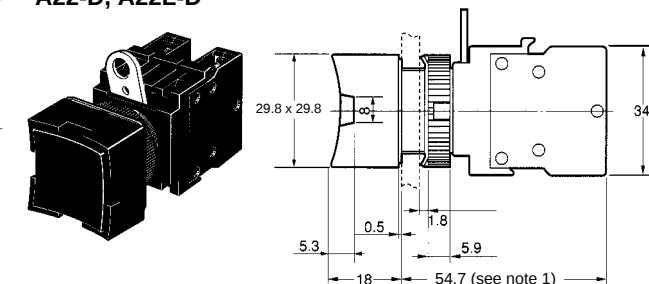
Square Full-guard Type A22-D, A22L-D
